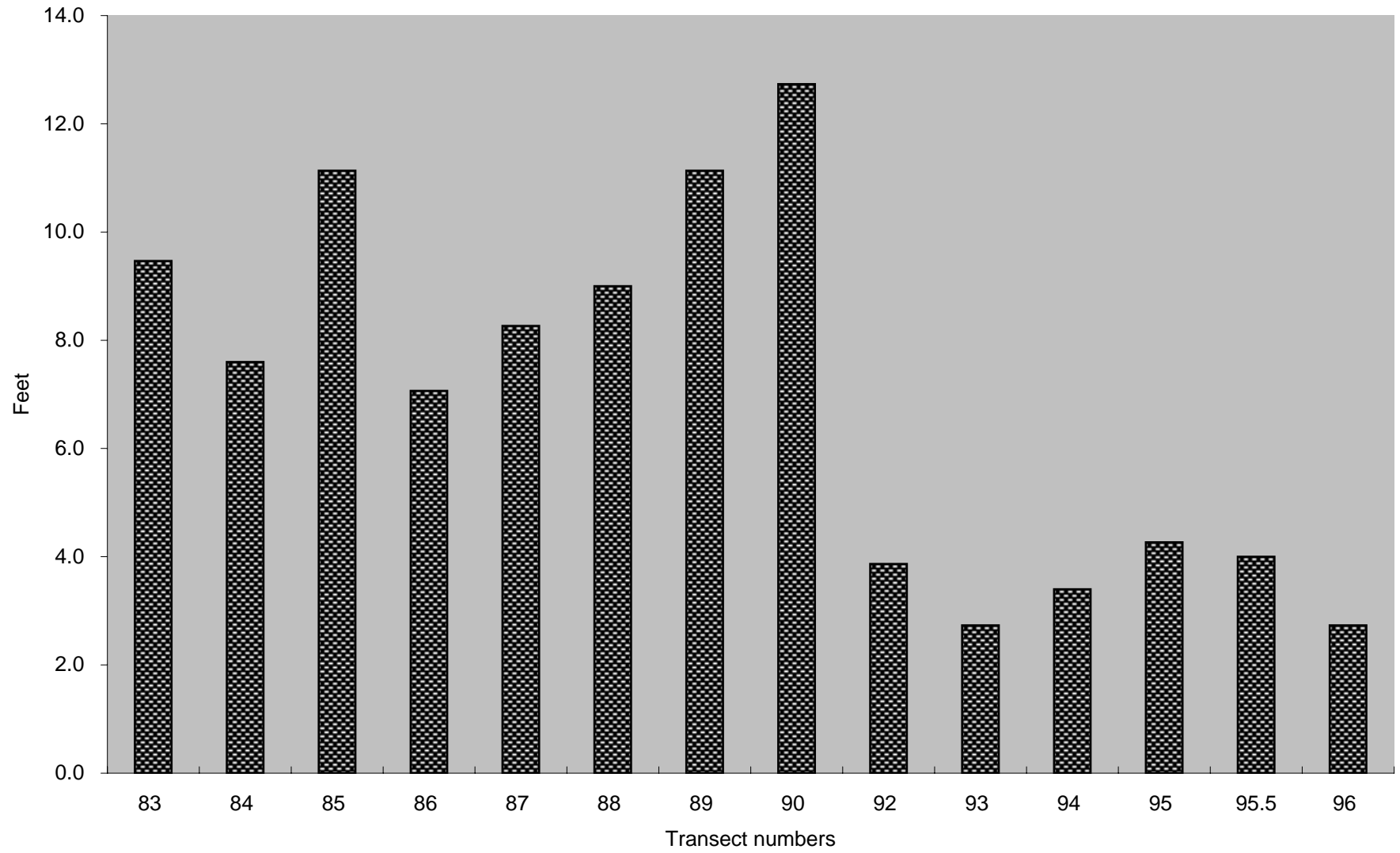
Avg. rate of erosion vs transect
